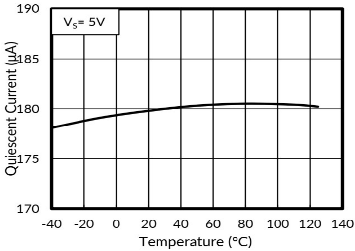
Figure 9. Quiescent Current vs Temperature
