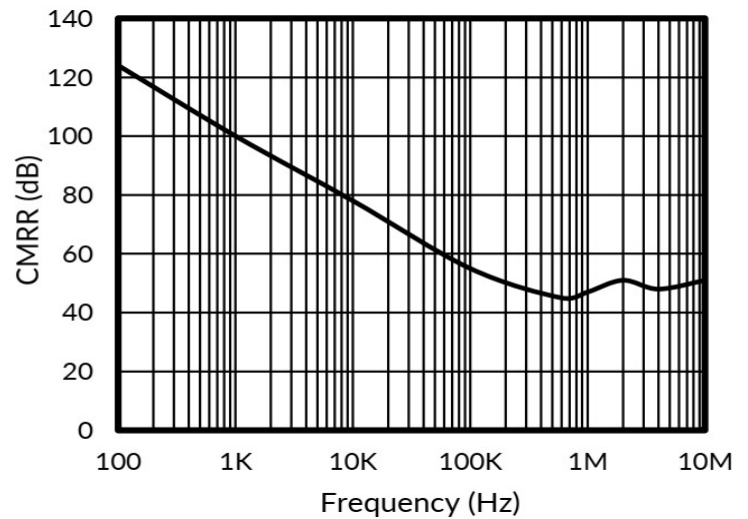
Figure 6. Common-Mode Rejection Ratio vs Frequency
