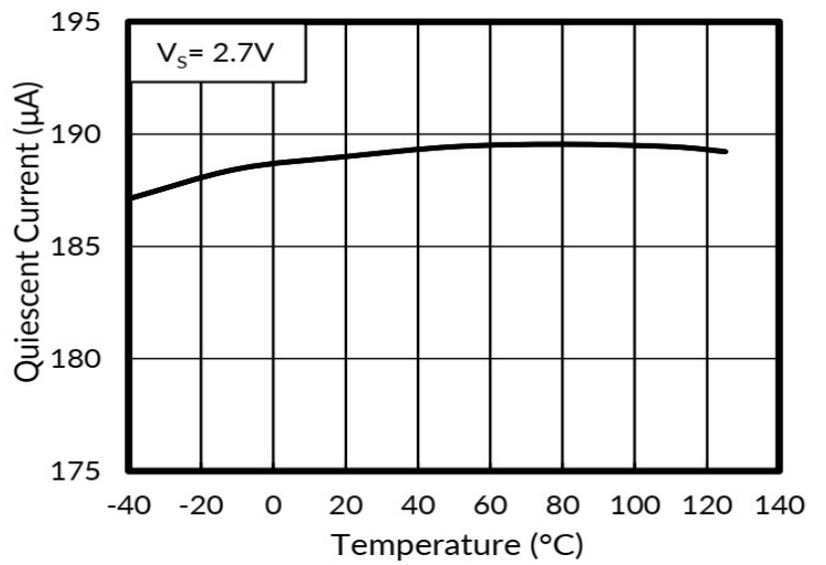
Figure 10. Quiescent Current vs Temperature
