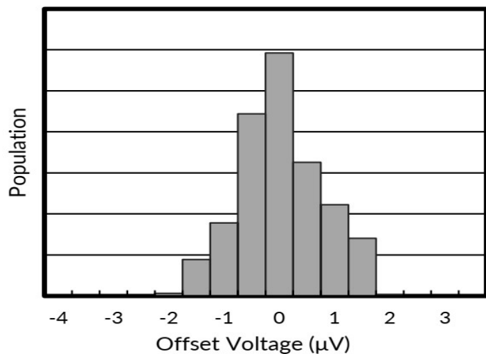
Figure 7. Offset Voltage Production Distribution
