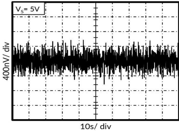
Figure 17. 0.01Hz to 10Hz Noise
