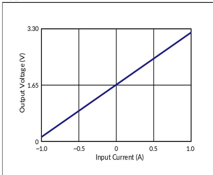
Figure 22. Bidirectional Current-Sensing Circuit Performance: Output Voltage vs Input Current
