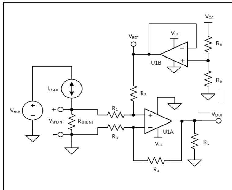
Figure 21. Bidirectional Current-Sensing Schematic
