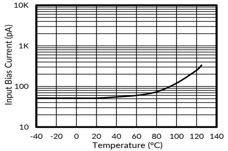
Figure 4. Input Bias Current vs temperature
