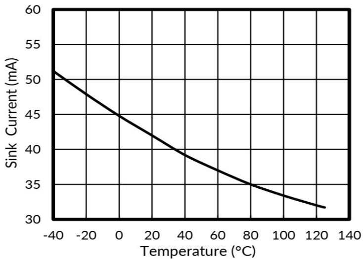
Figure 11. Sink Current vs Temperature
