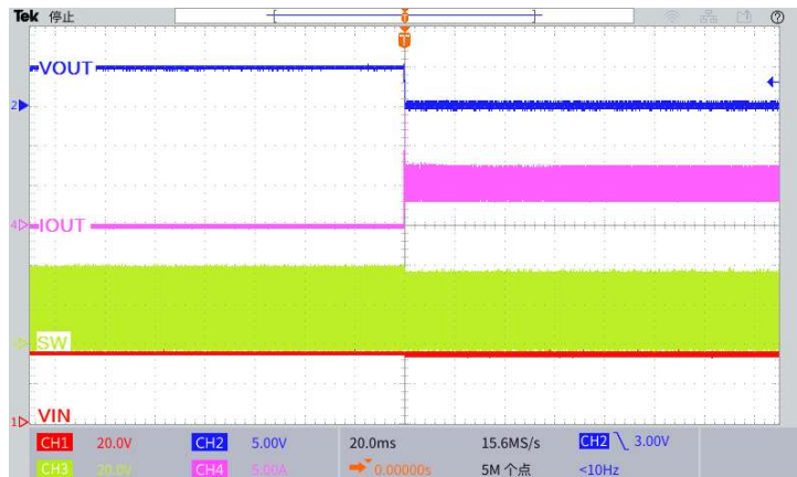
Figure 19. Output Short Circuit Waveform
