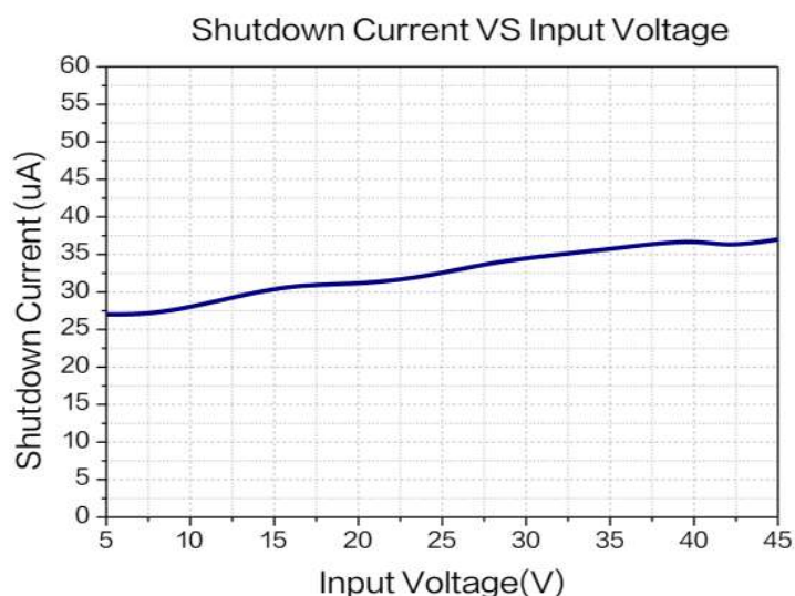
Figure 5. Shutdown Current
