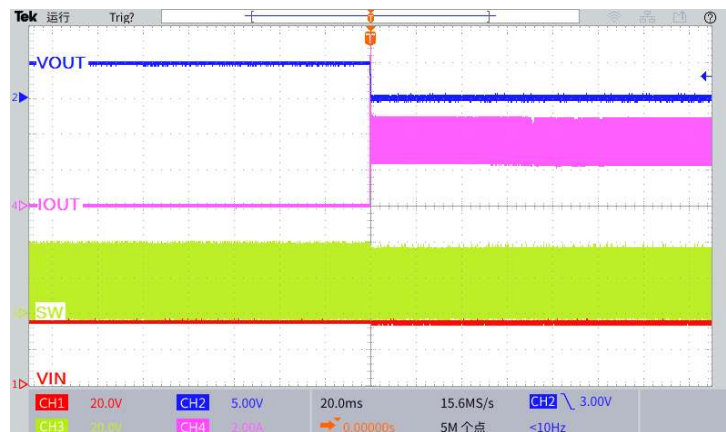
Figure 20. Output Short Circuit Waveform
