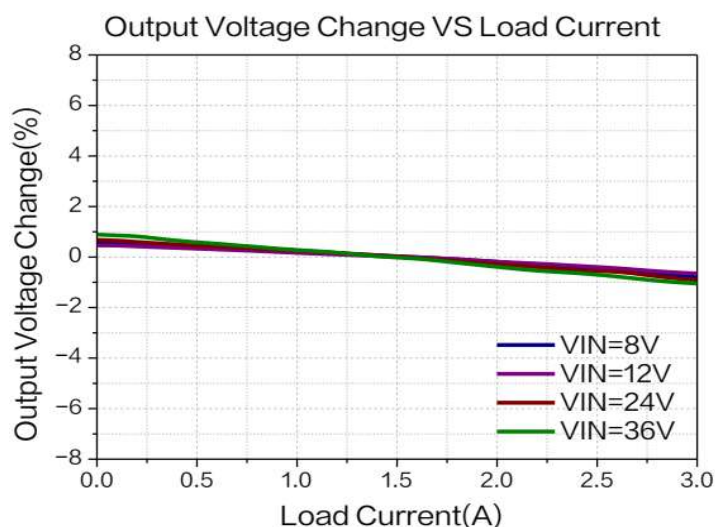
Figure 4. Load Regulation
