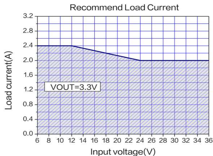
Figure 9. Max. Output Current
