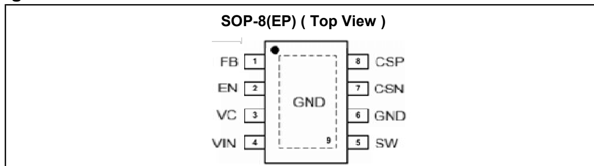
Figure 2. Pin Configuration of HCR3323 (Top View )
