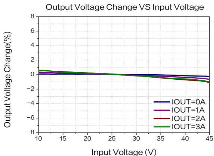
Figure 3. Line Regulation
