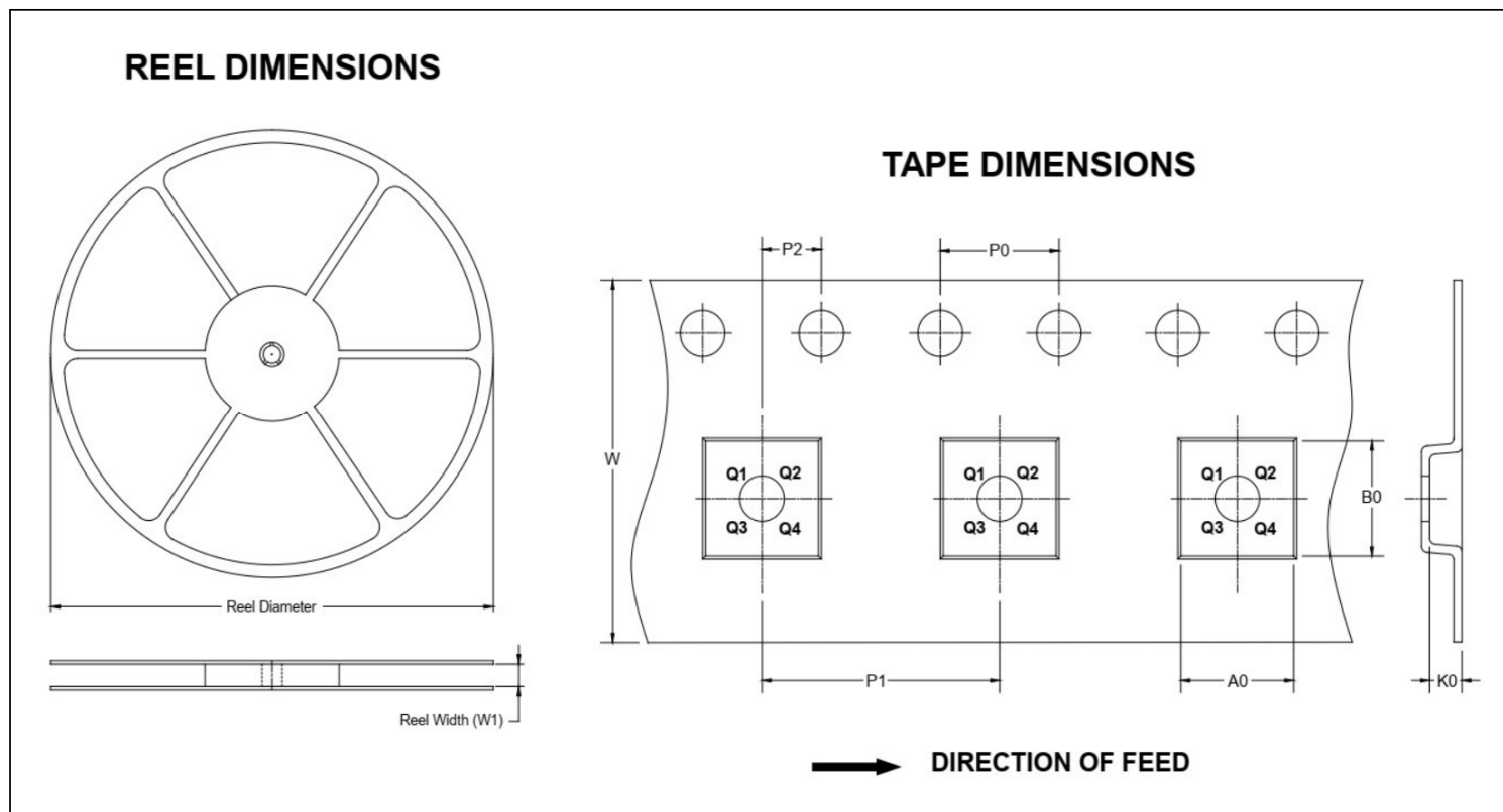
Reel and Tape Dimensions
