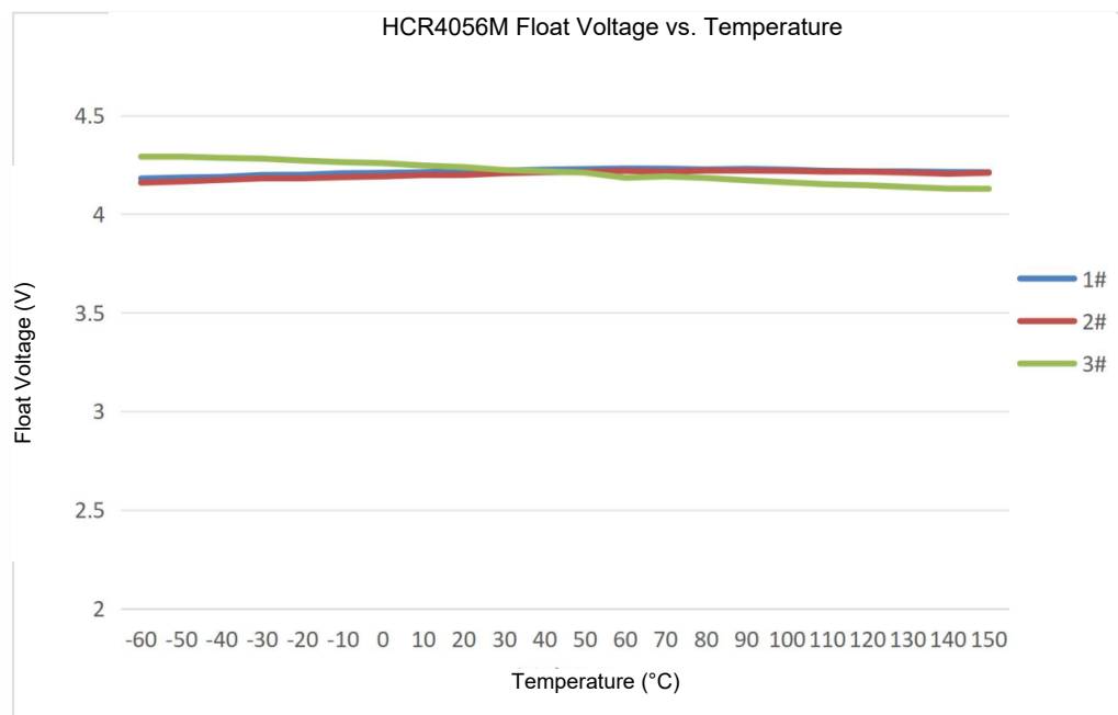
Figure 8. Float Voltage vs. Temperature ( V_{IN} = 5V , PROG = 5.1k\Omega )
