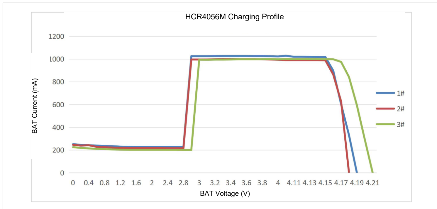
Figure 6. Charging Curve ( V_{IN} = 5V , PROG = 1.2k\Omega )
