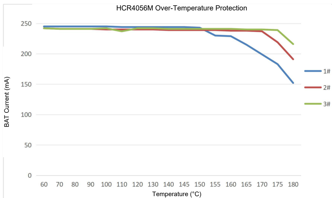
Figure 9. Overtemperature Protection ( V_{IN} = 5V , PROG = 2k\Omega )
