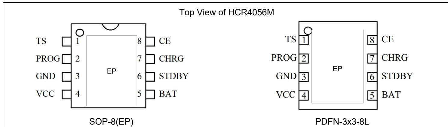
Figure 2. Pin Configuration of HCR4056M
