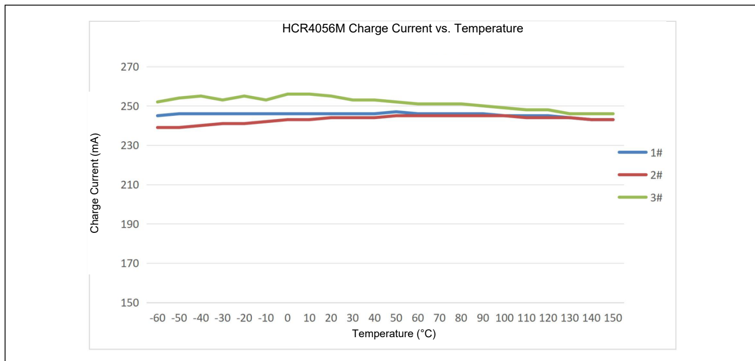
Figure 7. Charging Current vs. Temperature ( V_{IN} = 5V , PROG = 5.1k\Omega )
