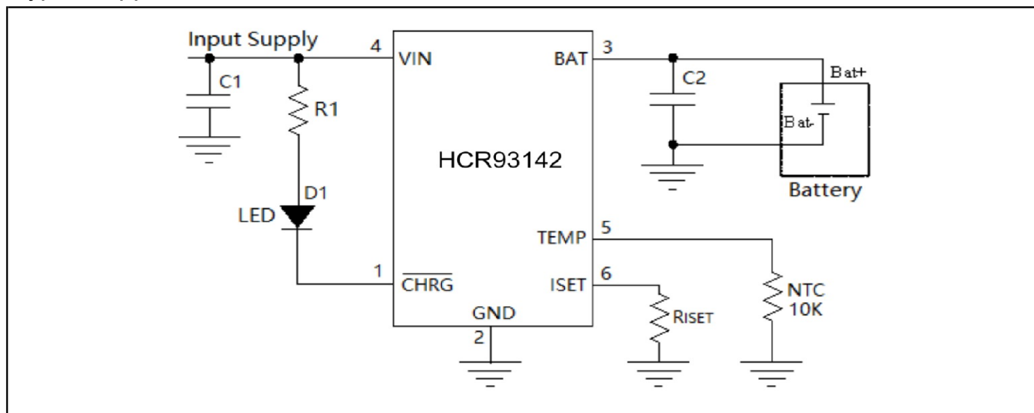
Figure 4. Typical Application Circuit
