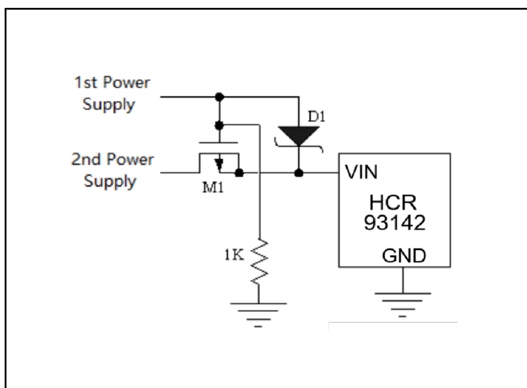
Figure 6. Combining 2 Input Power Supply
