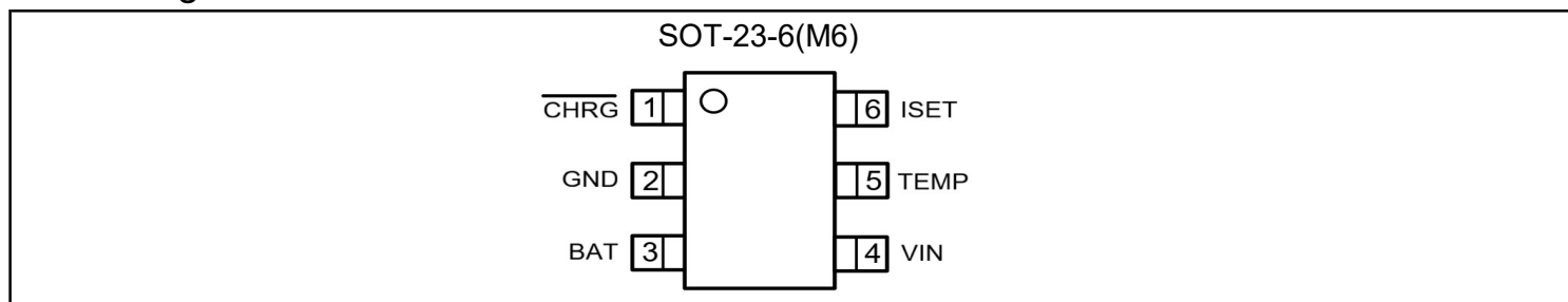
Figure 2. Pin Configuration of HCR93142 (Top View )
