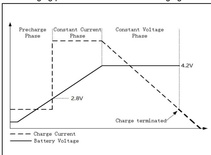
Figure 5. Charging Profile
