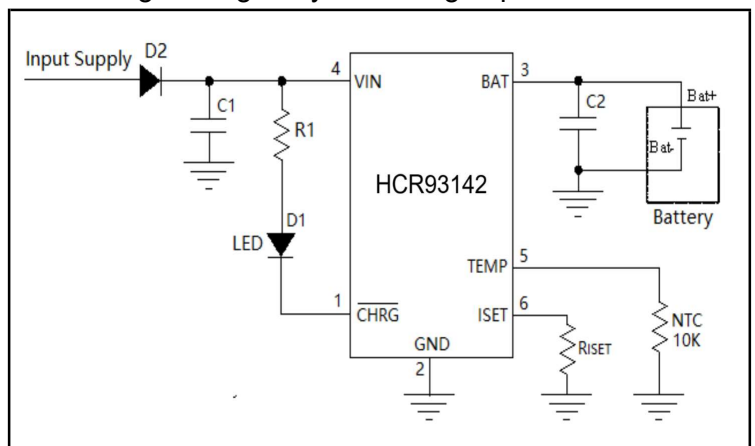
Figure 7. Adding Diode D2 to Suppress Voltage Spike
