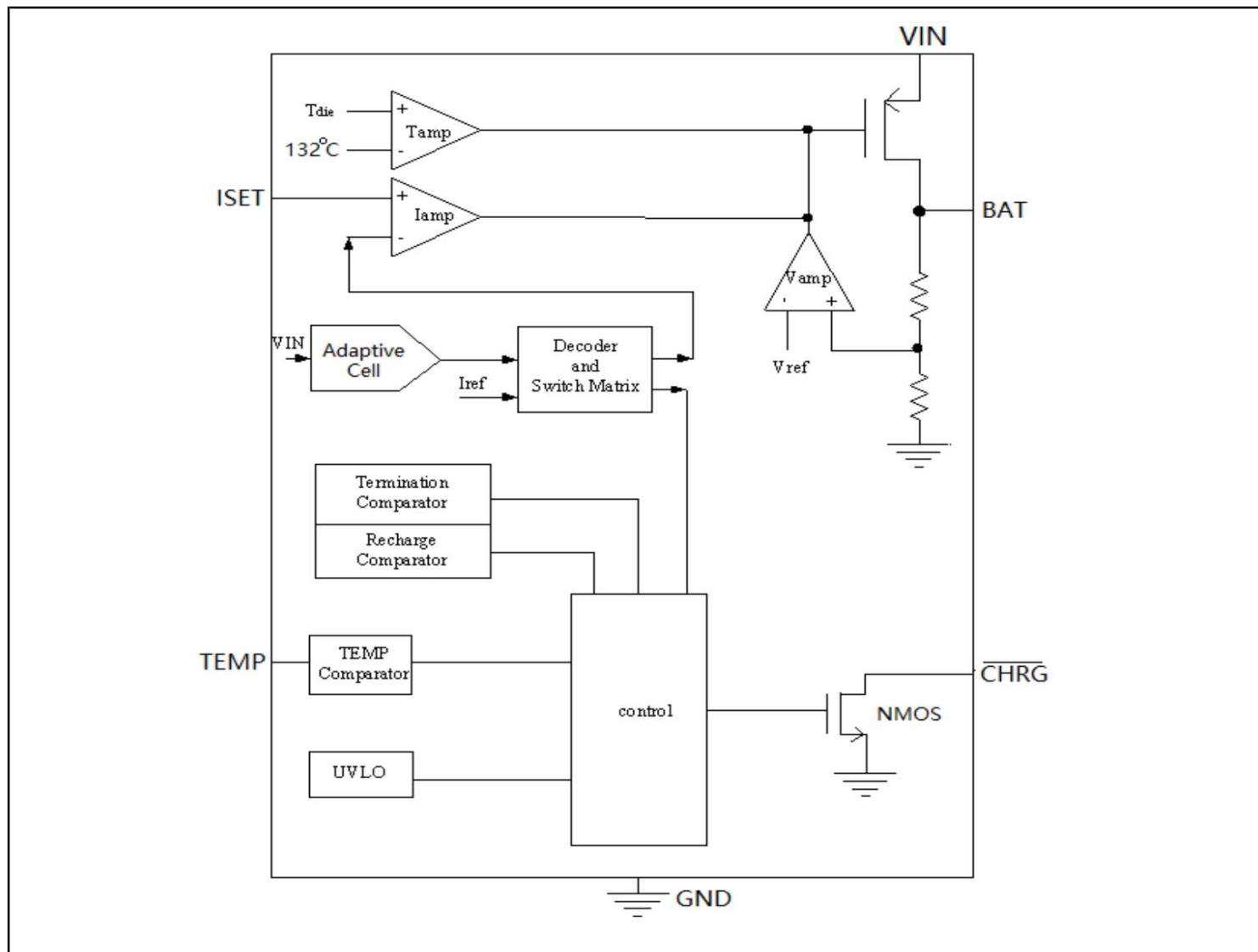
Figure 3. Functional Block Diagram
