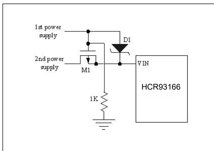
Figure 8. Combining 2 Input Power Supply
