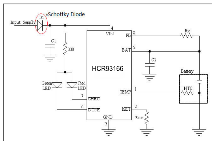
Figure 9. Adding Diode D1 to Suppress Voltage Spike
