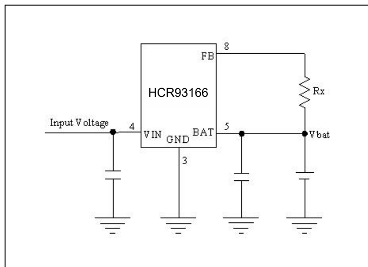
Figure 7. Adjusting Regulation Voltage in Constant Voltage Mode
