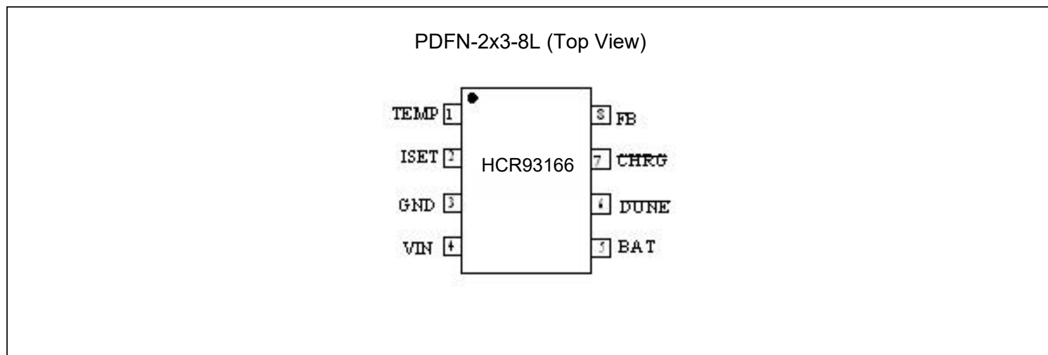
Figure 2. Pin Configuration of HCR93166
