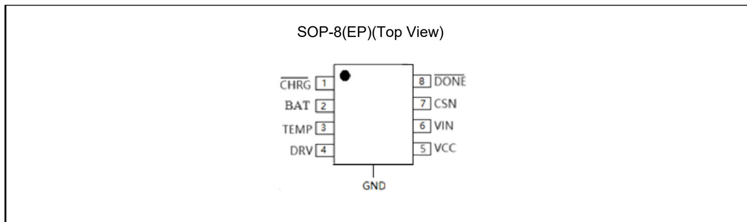
Figure 2. Pin Configuration
