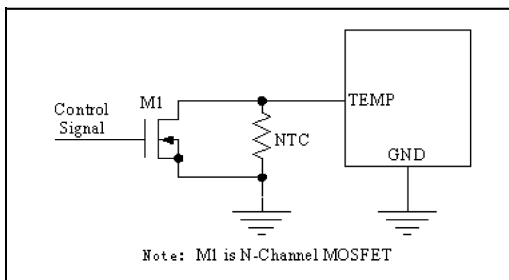
Figure 6. Disable Charging With TEMP Pin
