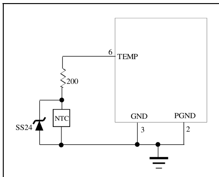
Figure 5. Using Battery Temperature Monitoring Function
