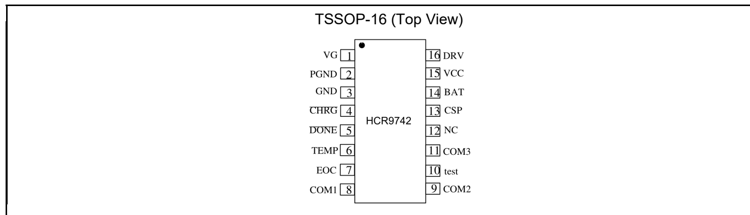
Figure 2. Pin Configuration
