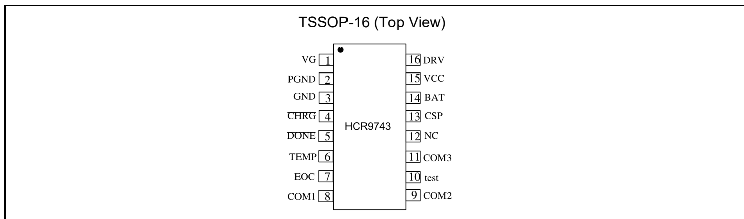
Figure 2. Pin Configuration
