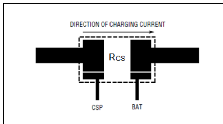
Figure 7. Kelvin Sensing of Charge Current
