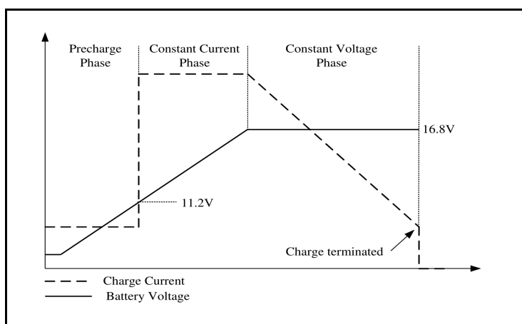
Figure 4. The Charging Profile
