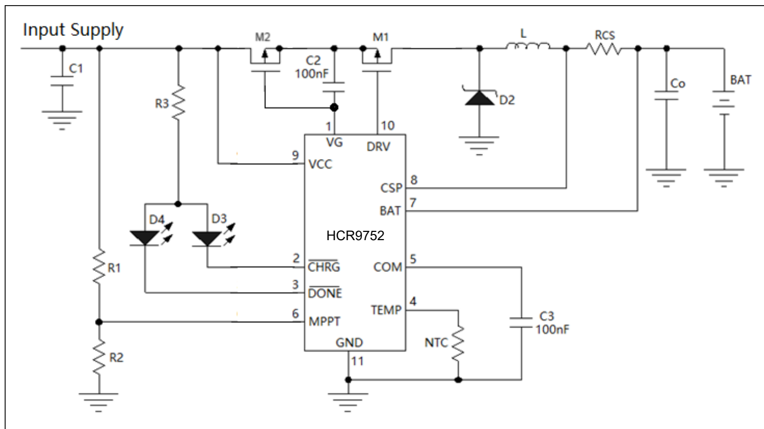
Figure 5. P-channel MOSFET to Block Battery Current Flowing back
