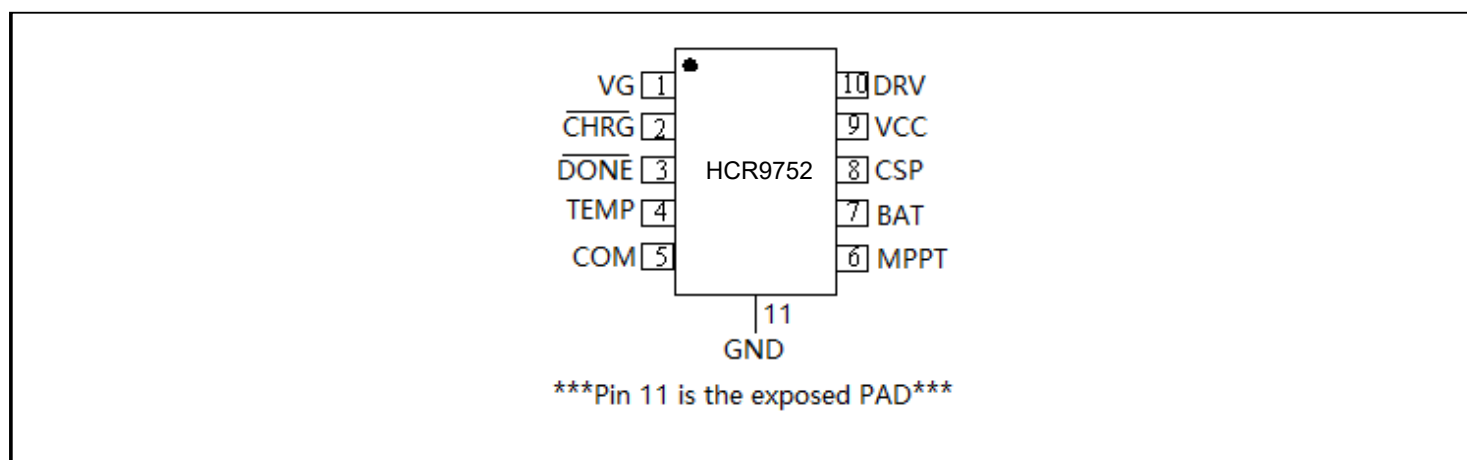
Figure 2. Pin Configuration (Top View)
