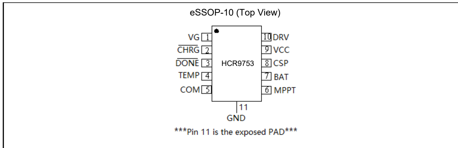
Figure 2. Pin Configuration
